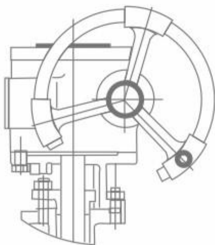
蜗轮传动 Worm gear operation
